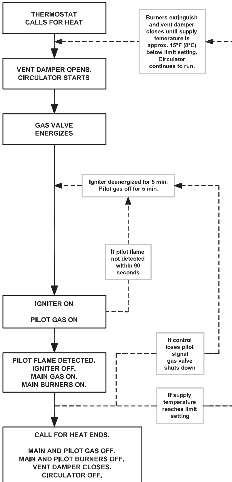
Figure 4: Intermittent Ignition Sequence of Operation
