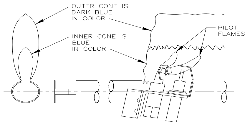
Figure 5: Intermittent Ignition Pilot Configuration and Flames
