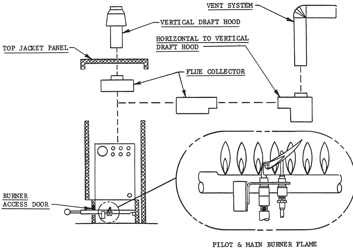
Figure 3: Boiler Components
