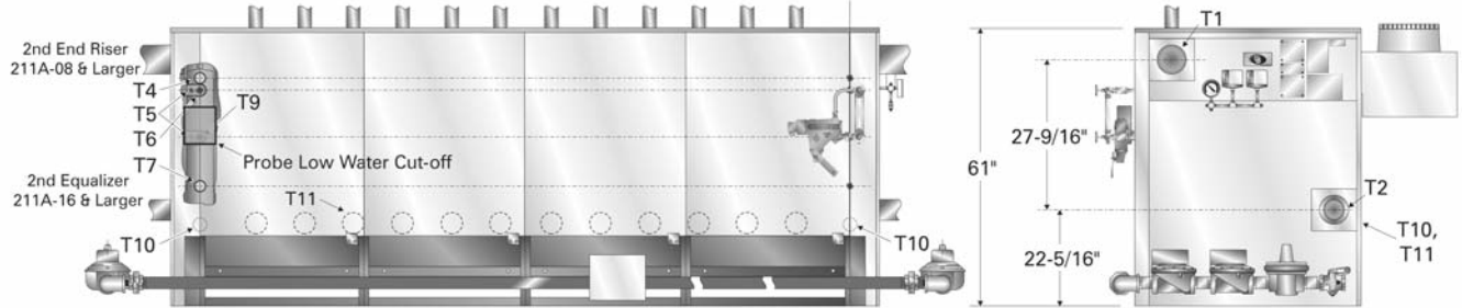
FRONT VIEW
