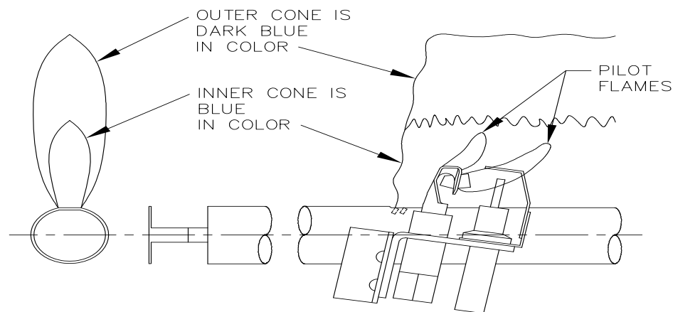
Figure 3: Pilot and Main Burner Flames
