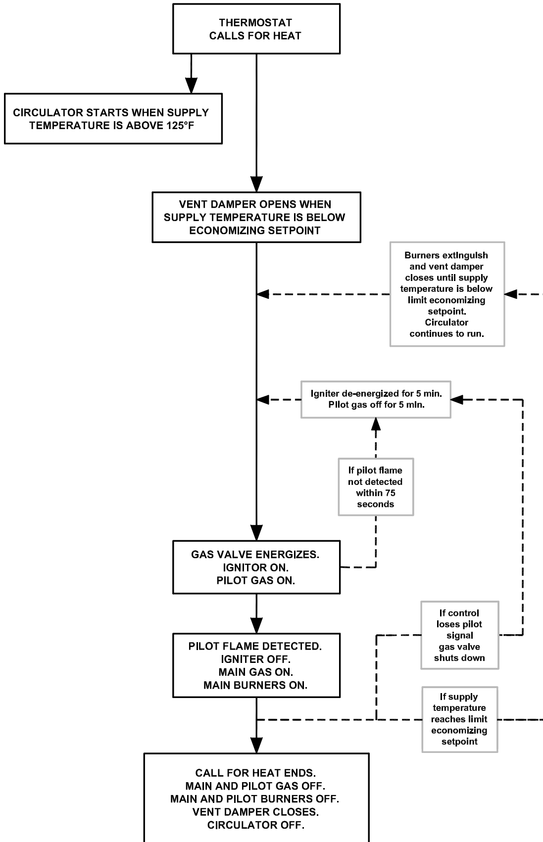
Figure 4: Intermittent Ignition Sequence of Operation
